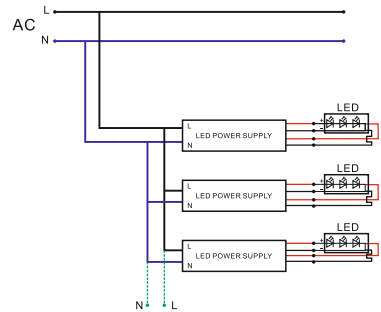
LED POWER SUPPLY
